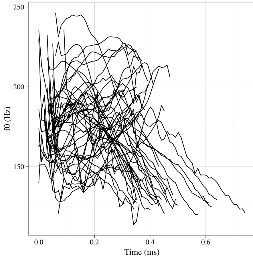
Figure 1: f0 contours from all recorded elicitation items from 20111207-1-kiy-ap-wordlist and 20111207-2-kiy-ap-framedwordlist.
